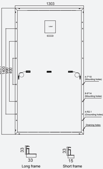
Back View
